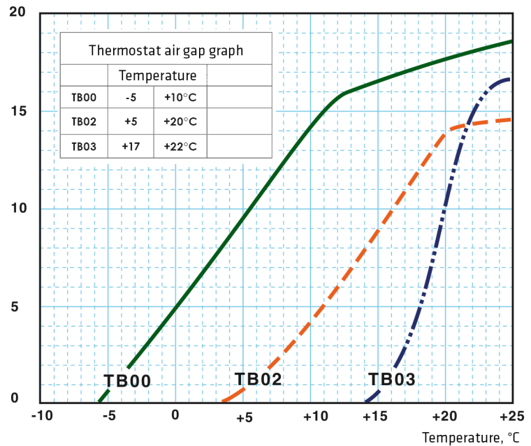
Air flow gap, mm
